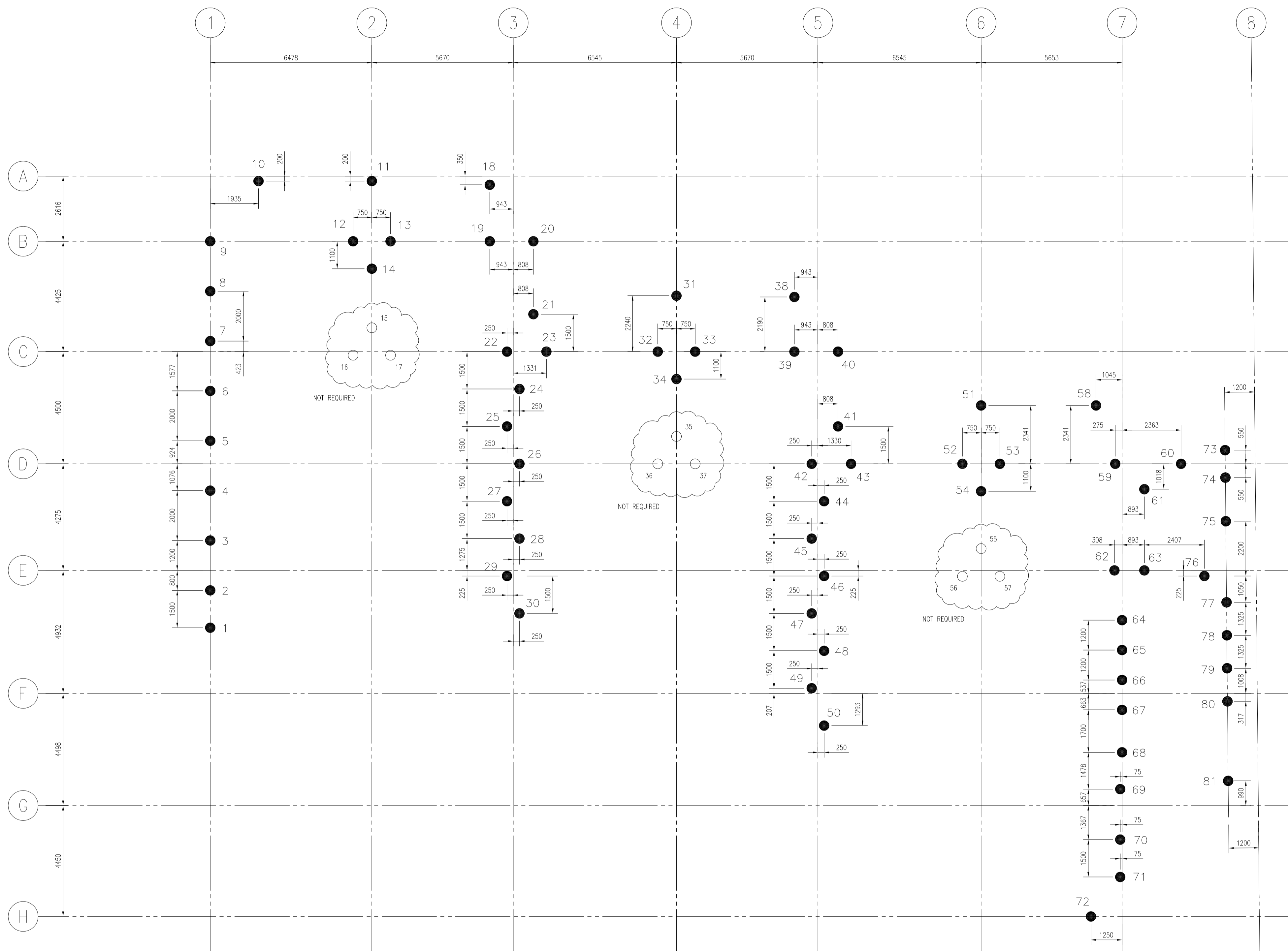
PILE LAYOUT (1:100)
